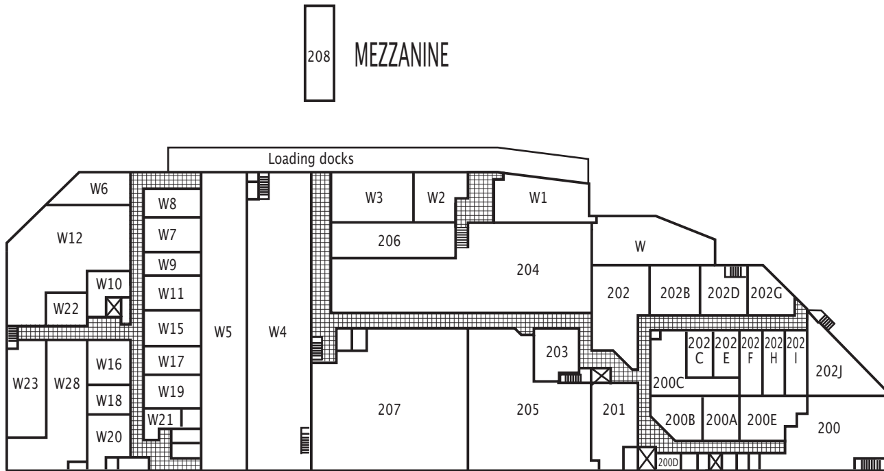
SECOND FLOOR
